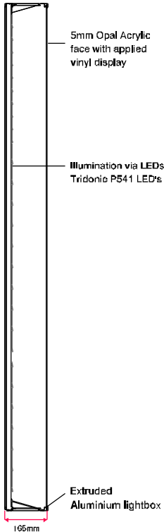
SECTION THROUGH scale 1:20
