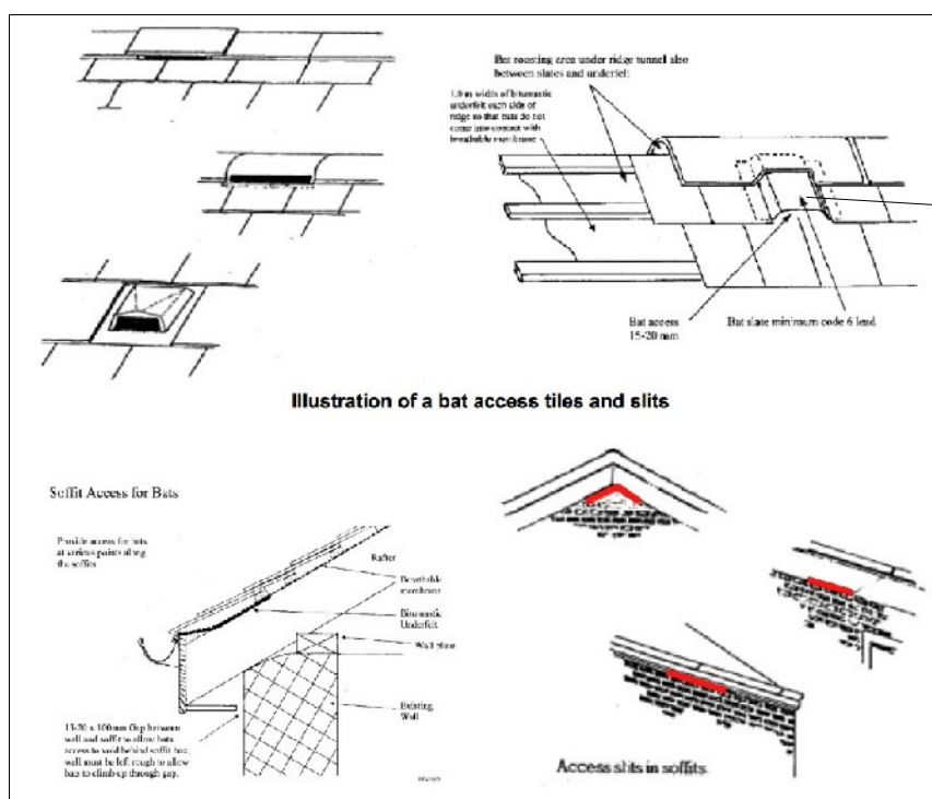
Fig.12. Examples of bat access tiles and soffit slits
