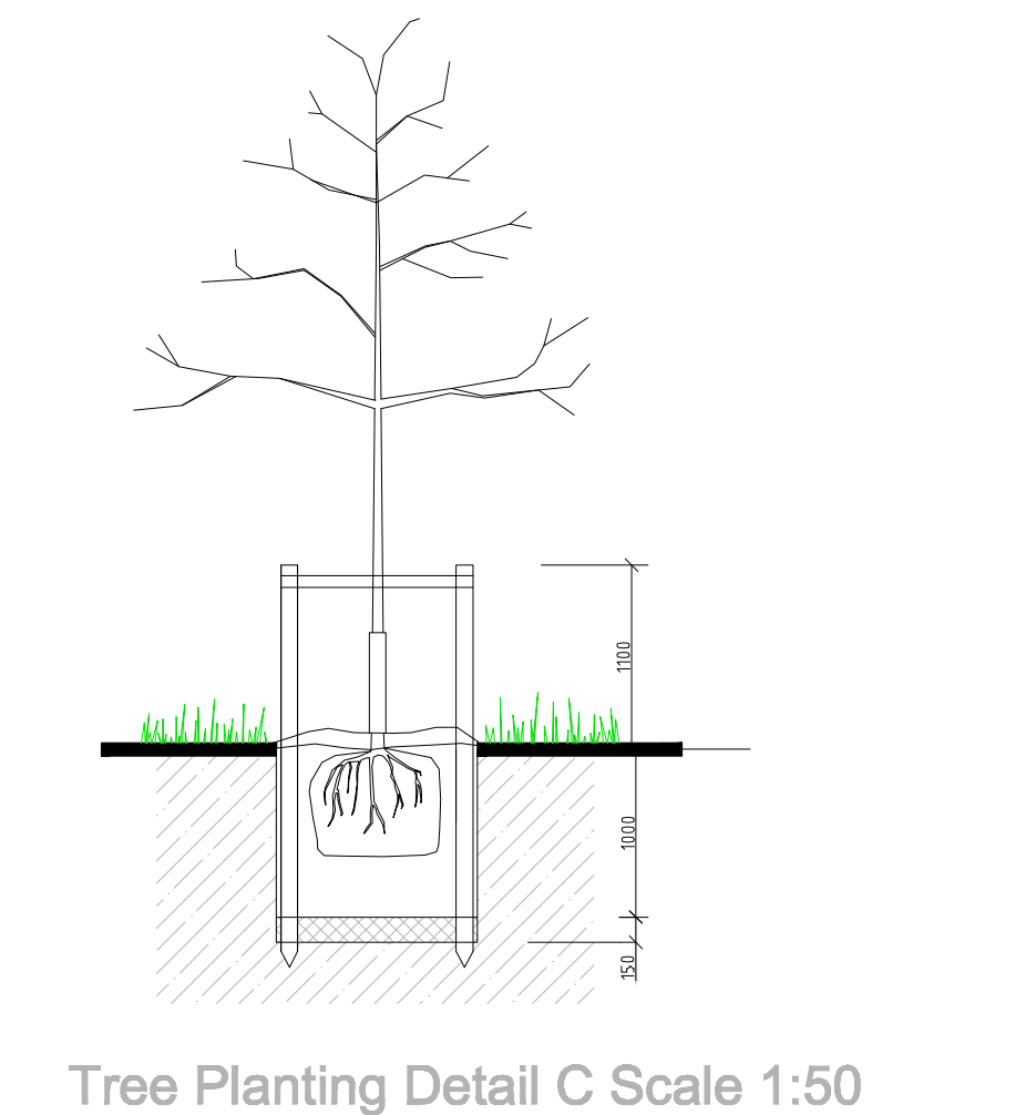
Tree Planting Detail C Scale 1:50
