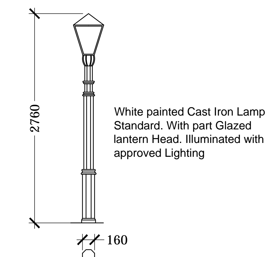
Lighting Standard Details 1:30
