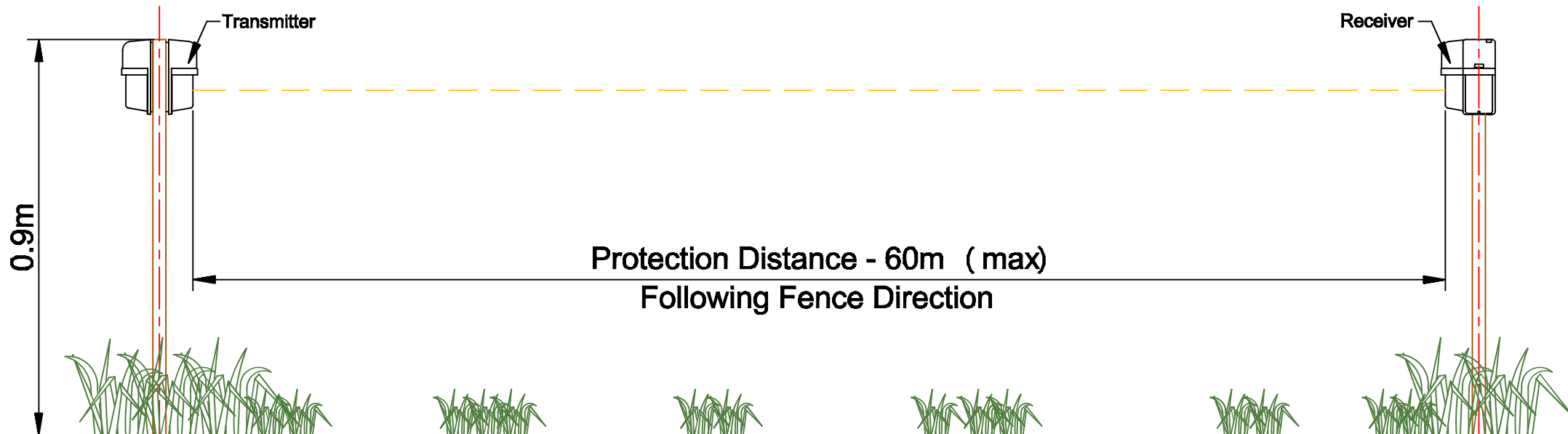
Photoelectric Beam Sensors Coverage Not To Scale
