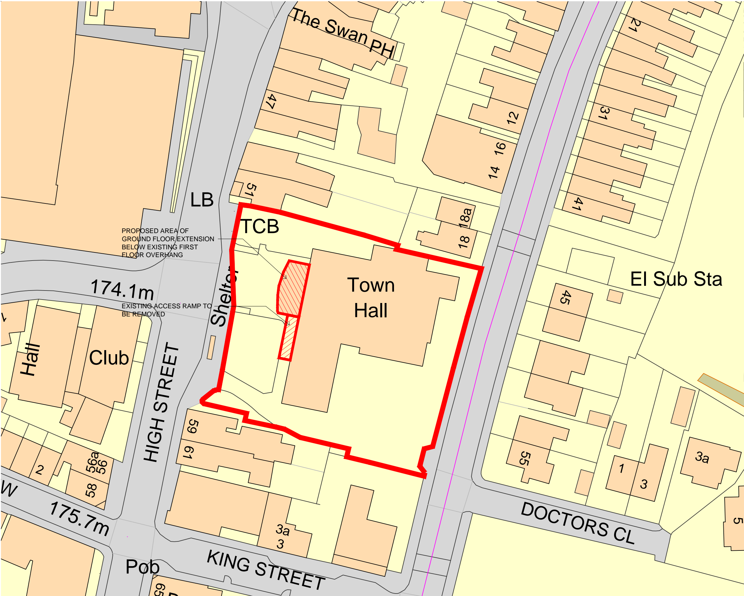
01 SITE PLAN A502 1:500 scale@A3 size
