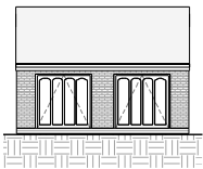
4 Elevation - Garage - Front 1 : 100
