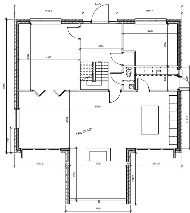
1 House Ground 1 : 50
