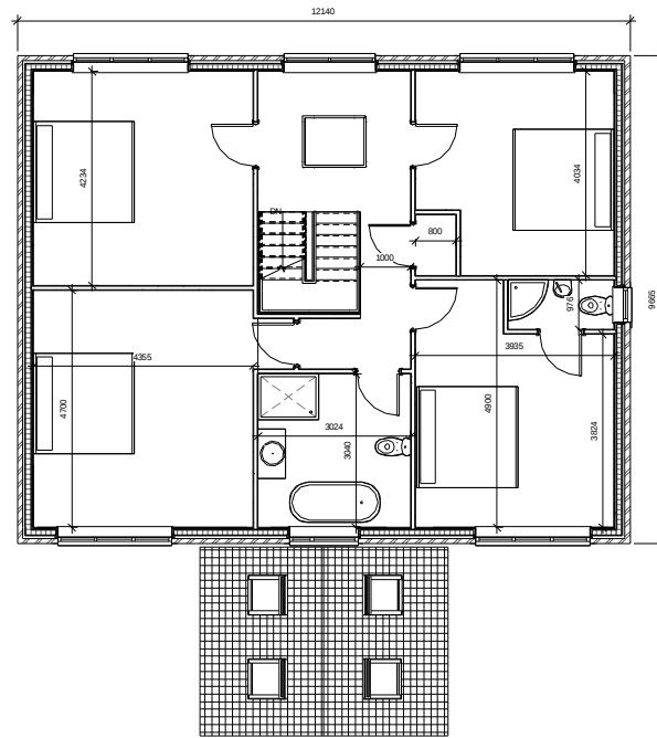
2 House Floor 1 1 : 50
